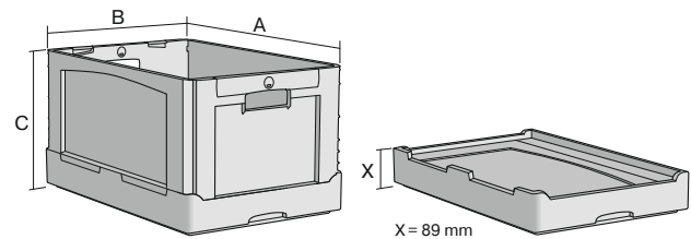
Pos. Dimensions, Tolerances as specified in DIN 16901
