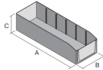
Pos. Dimensions, tolerances as specified in DIN 16901
