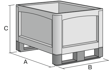
Pos. Dimensions, Tolerances as specified in DIN 16901
