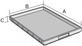
Pos. Dimensions, Tolerances as specified in DIN 16901
