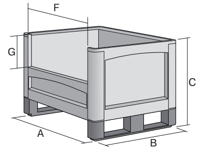
Pos. Dimensions, tolerances as specified in DIN 16901
